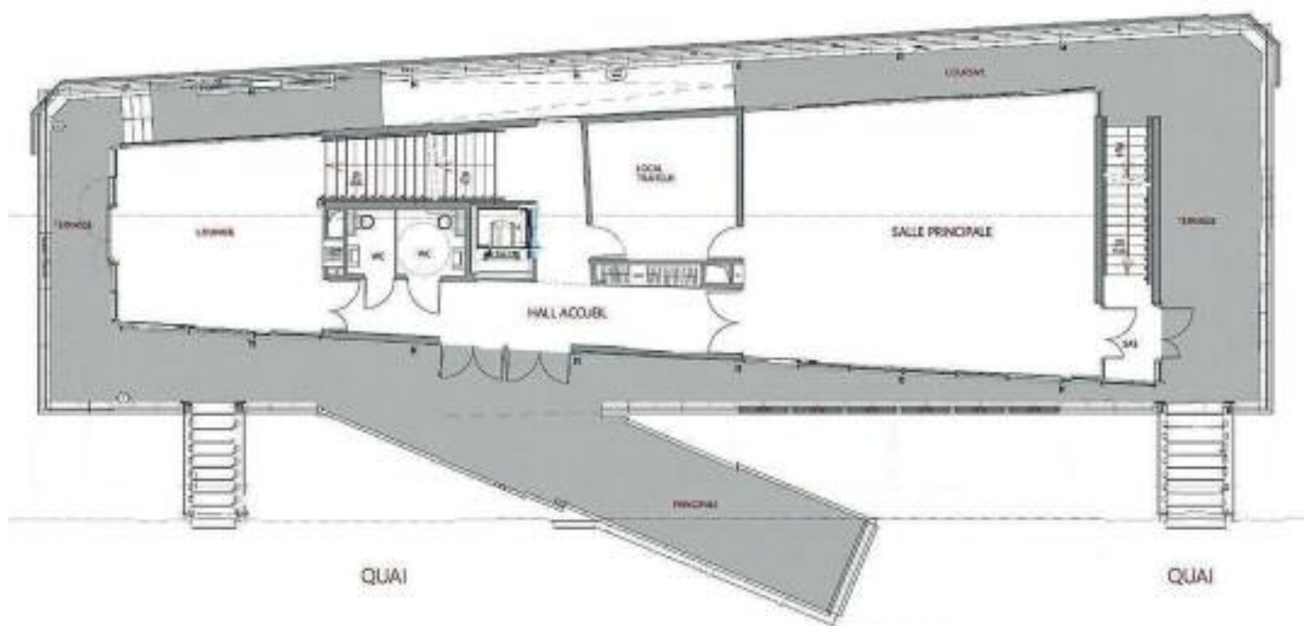
Plan pont principal / Main deck floorplan
